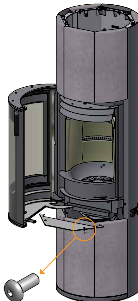
2 vis six pans RH M5x12
